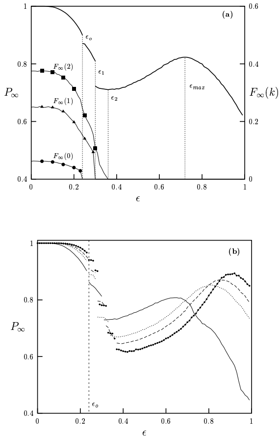
FIG. 3: (a) Left scale: Saturation persistence P_\infty as a function of \epsilon for the GSG embedded in Euclidean dimension d = 3 , represented by the thick dark line. The values \epsilon_o , \epsilon_1 , \epsilon_2 , and \epsilon_{max} are indicated by dotted vertical lines. Right scale: Fraction F_t(k) vs. \epsilon . Circles F_\infty(0) ; triangles F_\infty(1) ; squares F_\infty(2) . Lattice size is N = 4^9 . (b) P_\infty as a function of \epsilon for GSG embedded in different Euclidean dimensions d . Continuous line: d = 2 , N = 3^{11} ; dotted line line: d = 5 , N = 6^7 ; dashed line: d = 7 , N = 8^6 ; circle line: d = 11 , N = 12^5 . The first discontinuity at \epsilon_o = 0.24 , common to all lattices, is indicated.
